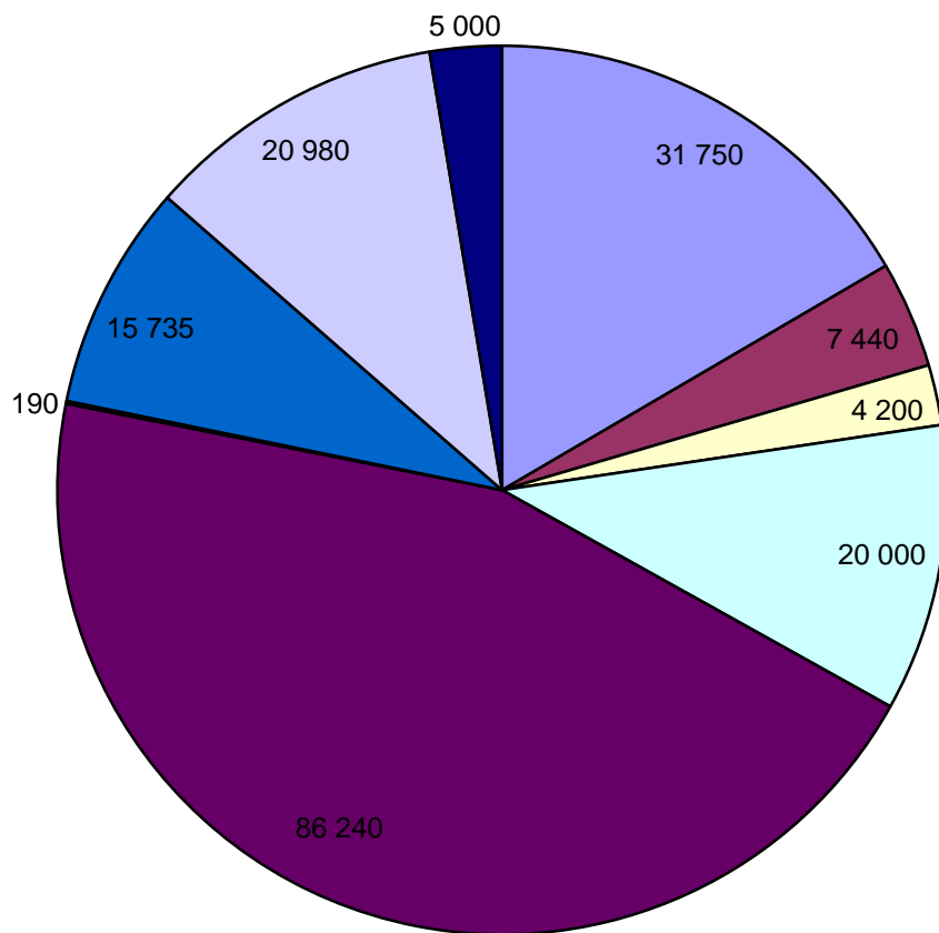
Operational costs of sludge composting plant [EUR/year], 3 900 m3 sludge / year
